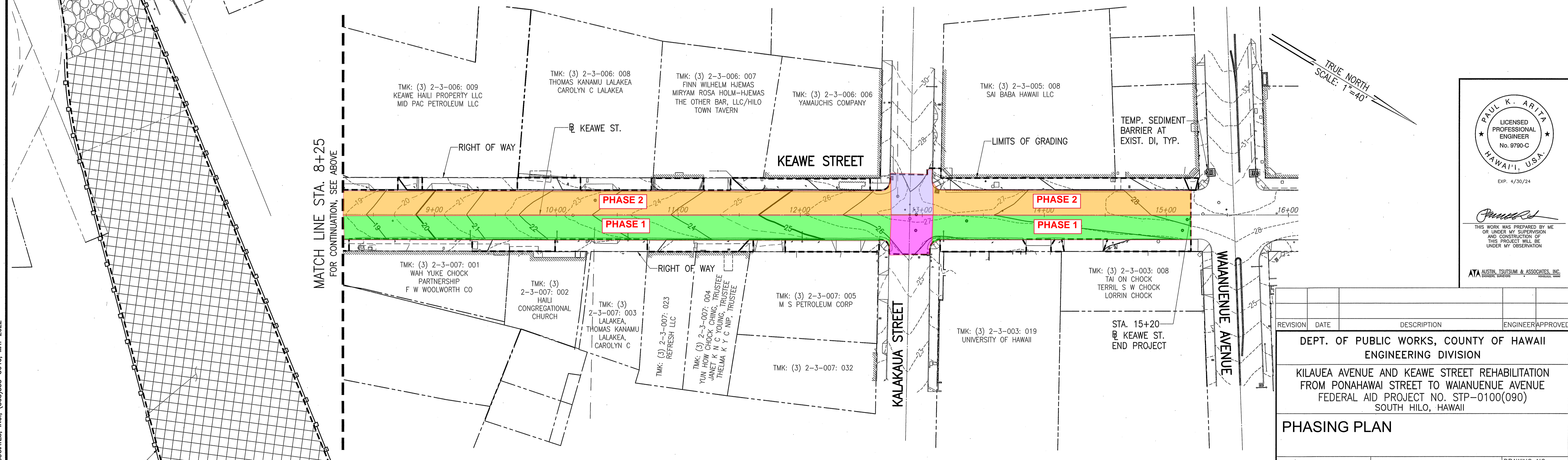
PHASING PLAN STA. 8+25 TO END SCALE: 1"=40'
