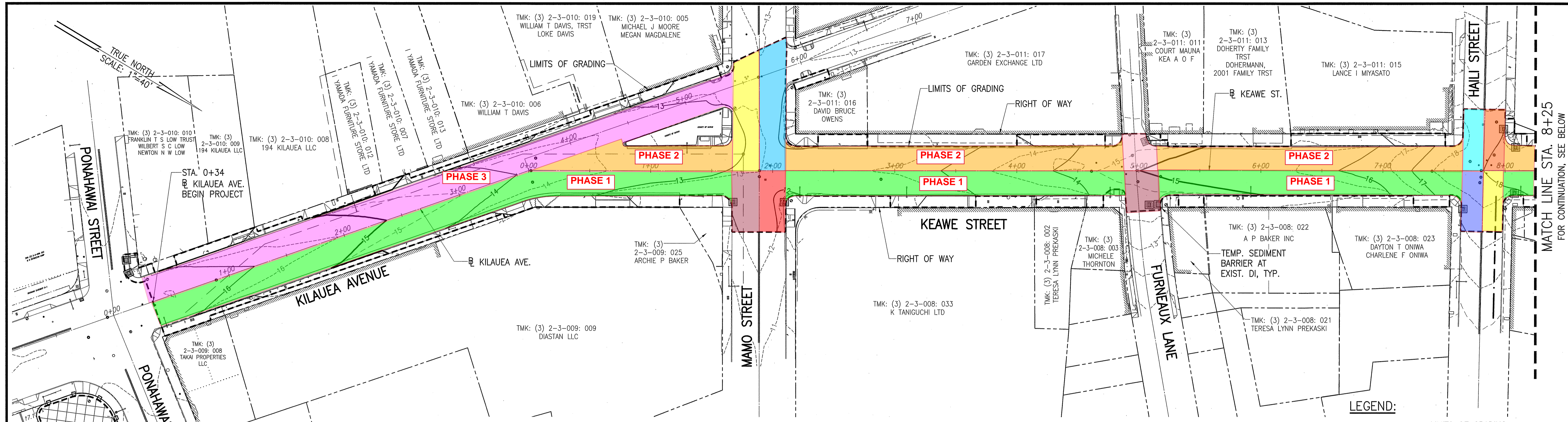
PHASING PLAN STA. 0+00 TO 8+25 SCALE: 1"=40'
