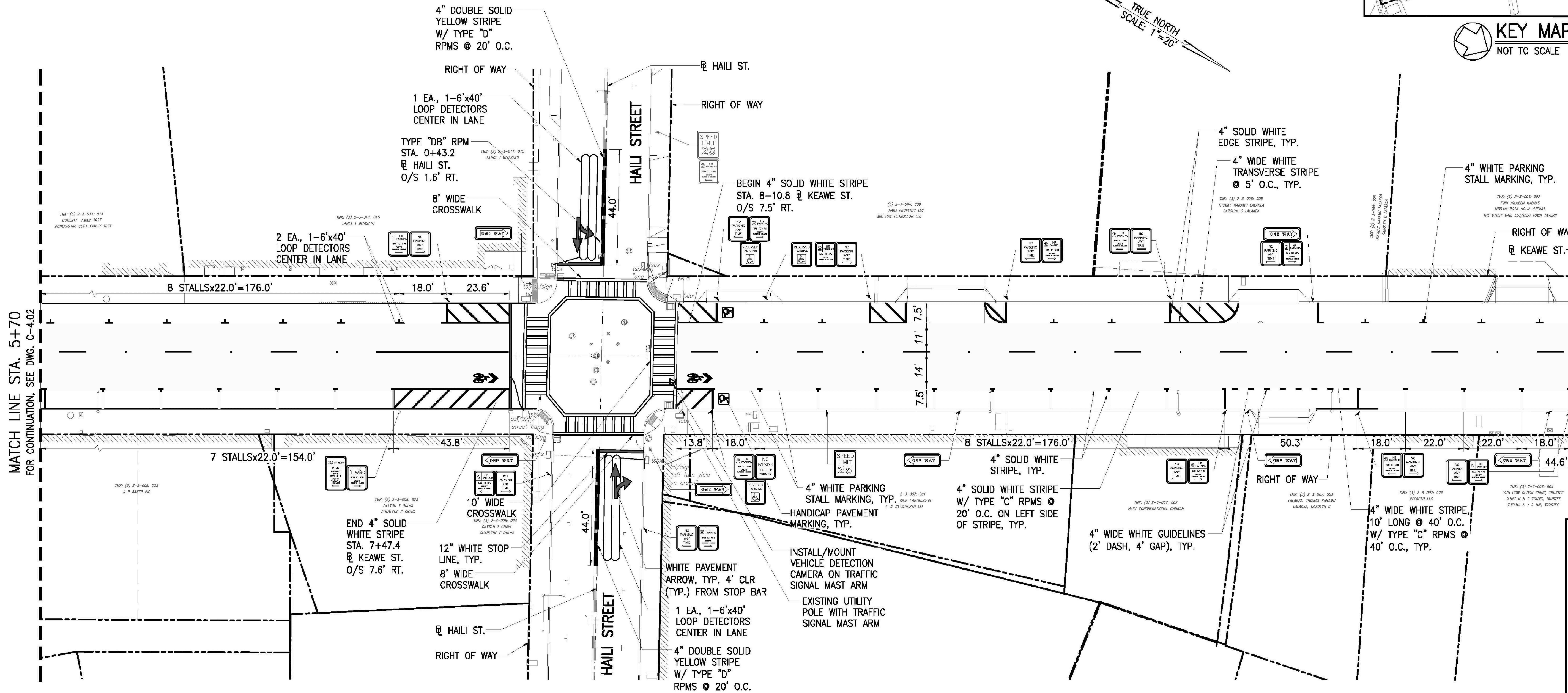
SIGNING AND STRIPING PLAN – 3 SCALE: 1"=10'
